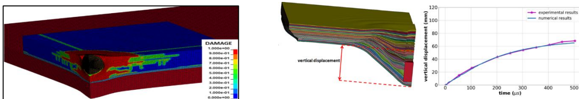
Figure 2 : Numerical model under rapid dynamic of the perforation of three-layer protection.
