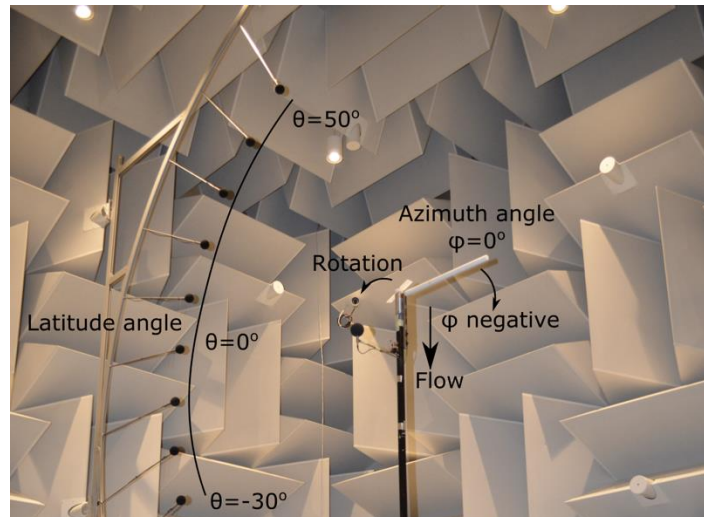
Figure 2: Photography of the experimental setup in ISAE-SUPAERO anechoic room.
